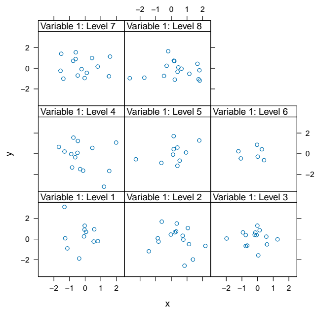
Figure 2: A lattice strip function using grid .
